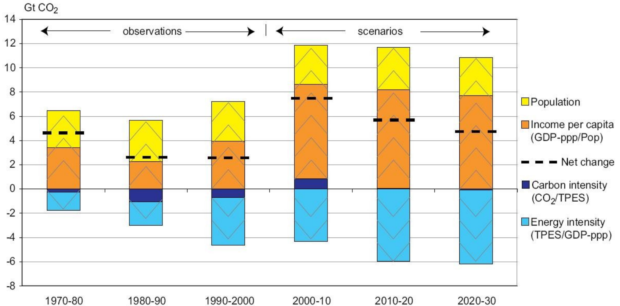
Figure 1.6: Decomposition of global energy-related CO 2 emission changes at the global scale for three historical and three future decades.
